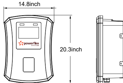
Enclosure
