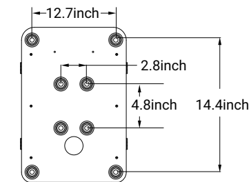
Wall-Mounted Bracket
