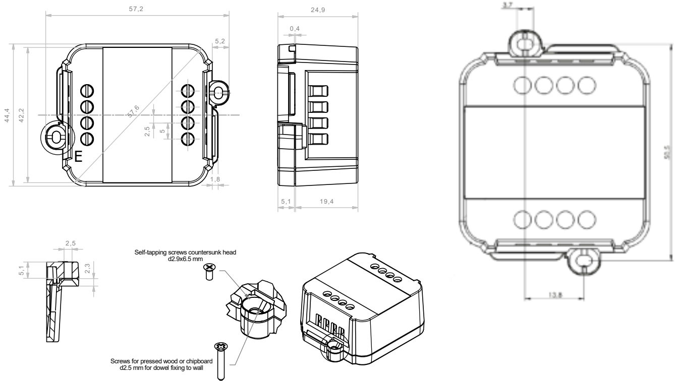
Figure 9: Mechanical dimensions
